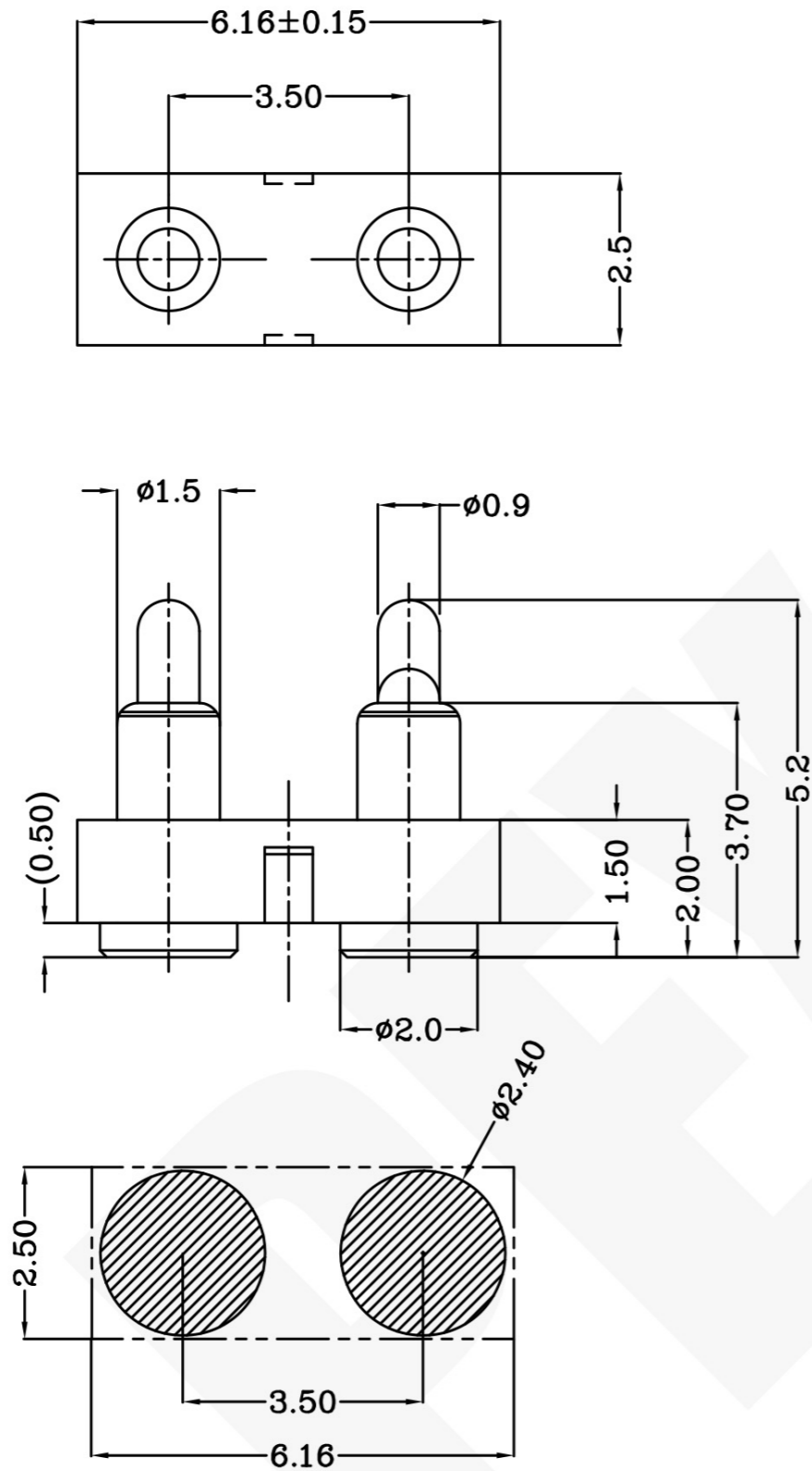
Recommended PCB Layout
