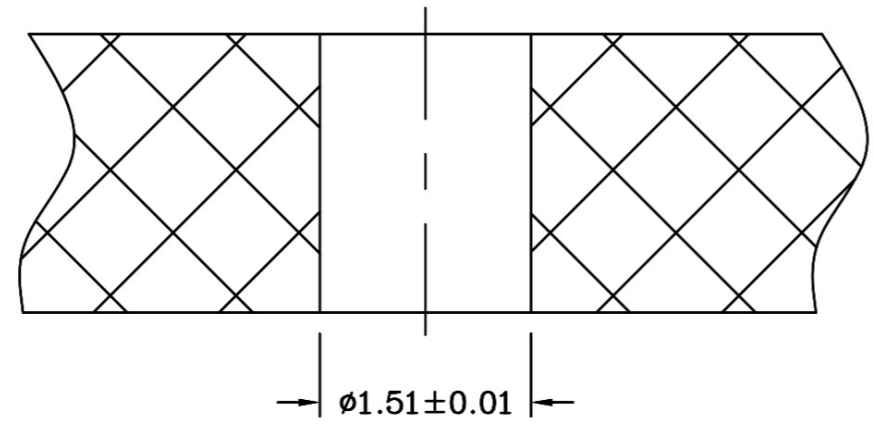
Recommended Dimensions of HSG
