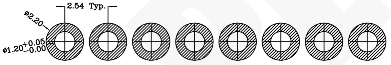
Recommended PCB Layout
